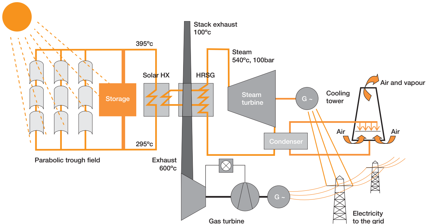
Figure 9: Integrated Solar/Combined Cycle System (ISCC)
