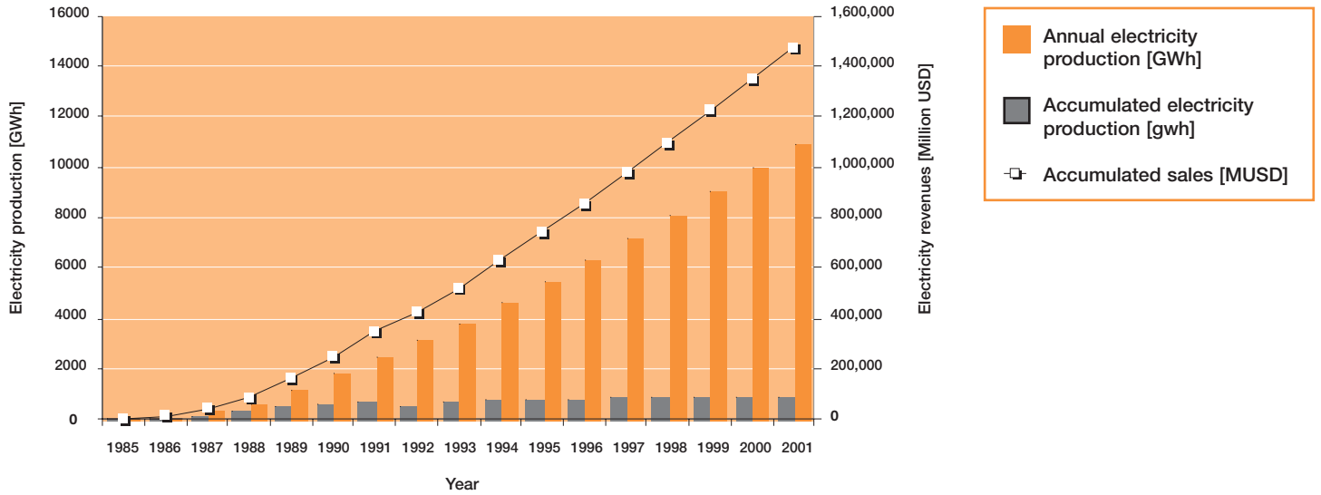
Figure 4: Electricity generation at Californian plants using parabolic trough collectors, 1985 to 2001
