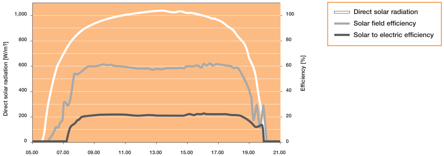
Figure 5: Daily summer output pattern at the SEGS VI plant in Kramer Junction, California
