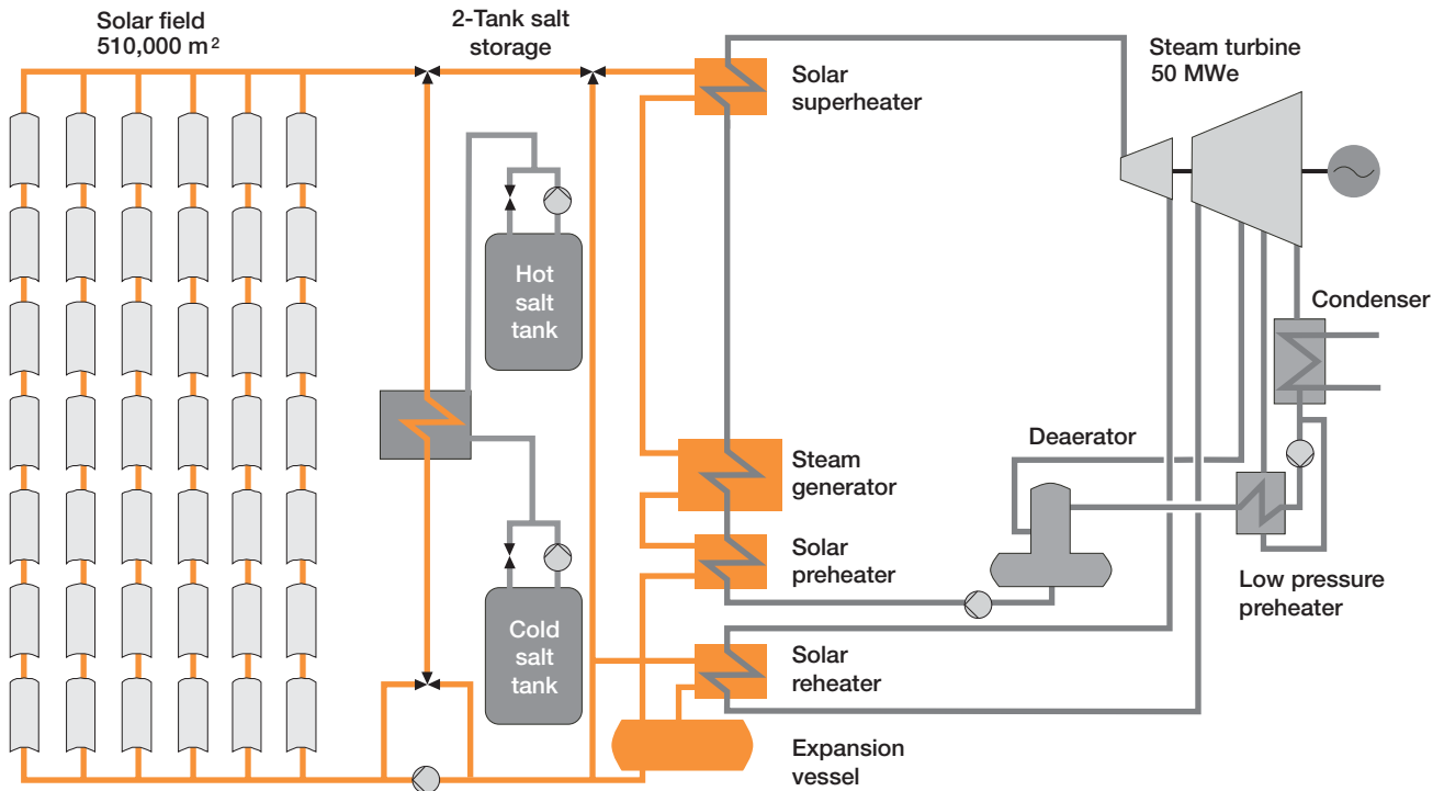
Figure 10: AndaSol Configuration diagrammatic scheme of the solar field, storage system and steam cycle at the AndaSol-1 project, southern Spain
