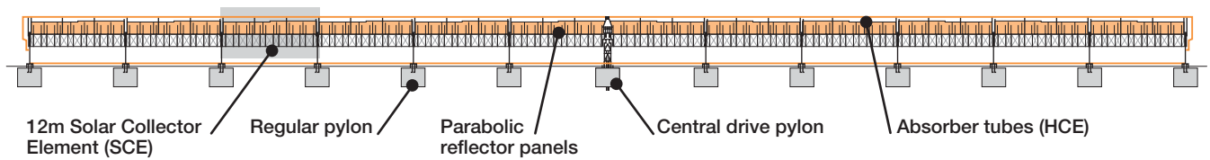
Figure 7: Side view of a EuroTrough ET150 collector unit (150m length)
