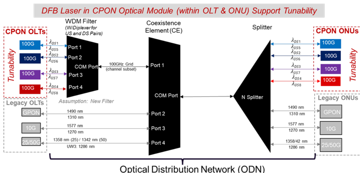
Figure 8. PON coexistence with single-splitter ODN
