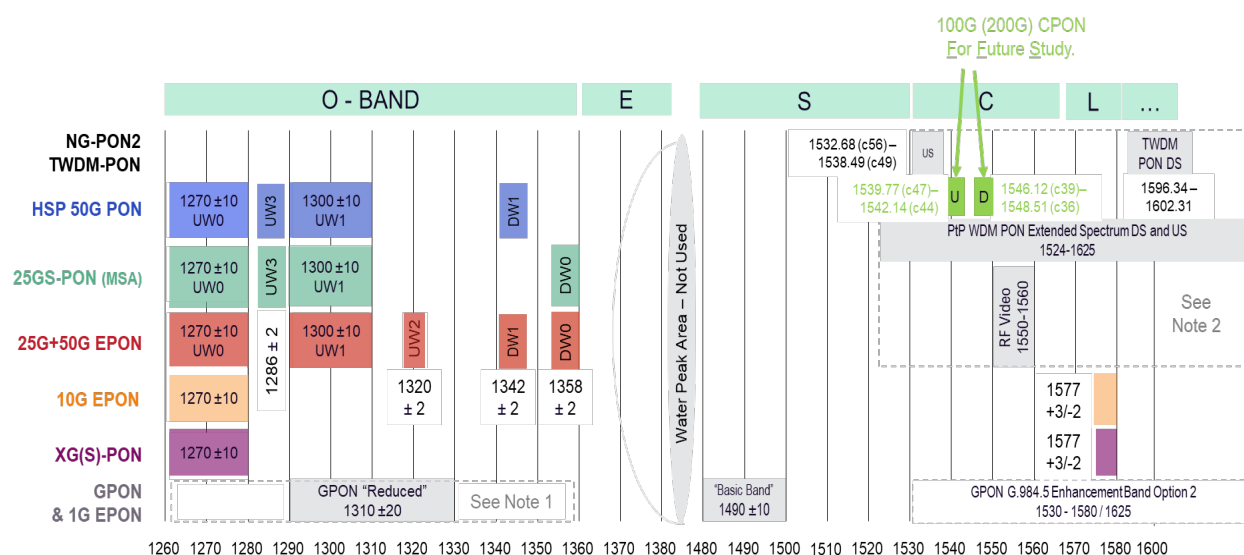
Figure 7. PON wavelengths
